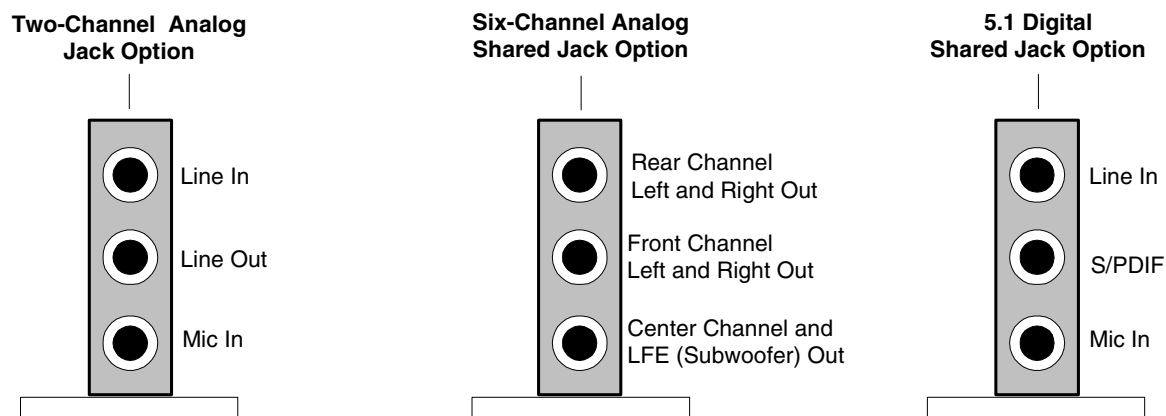
Figure 9. Back Panel Audio Connector Options for Flex 6 Audio Subsystem
